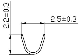
SEC C-C
