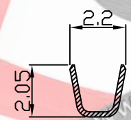
SEC B-B
