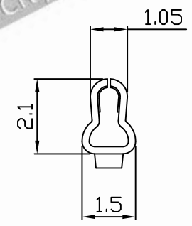
SEC C-C
