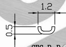
SEC B-B
