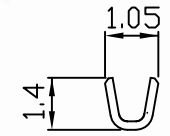
SEC C-C
