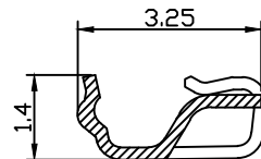
SEC B-B
