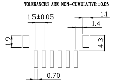
RECOMMENDED PCB LAYOUT (PCB THK=1.0~1.6)
