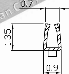
SEC C-C
